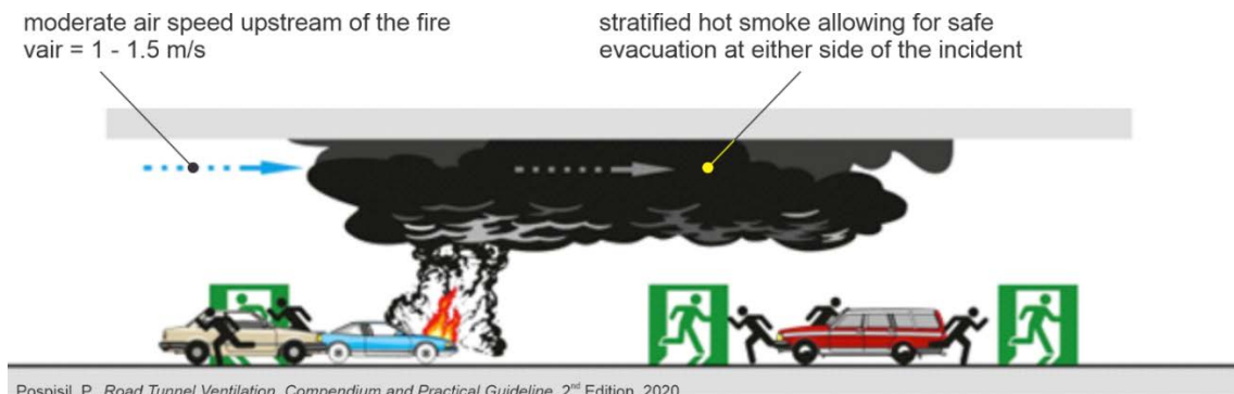
Figure 11 Longitudinal smoke control with low flow velocity (c.f., Pospisil 2020)
