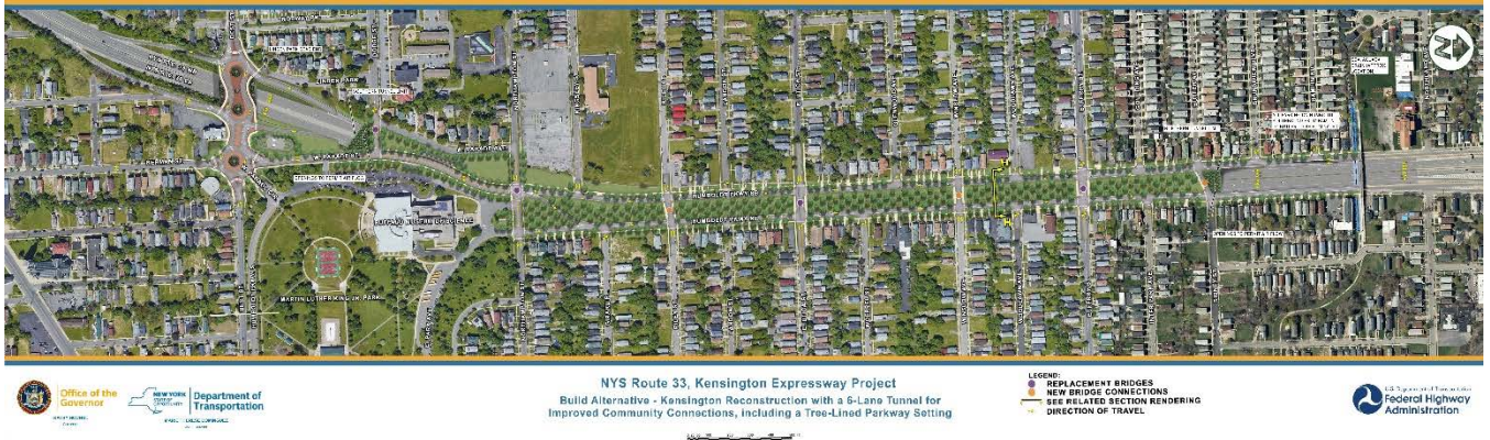
Figure 2 Kensington Expressway Capping Plan
